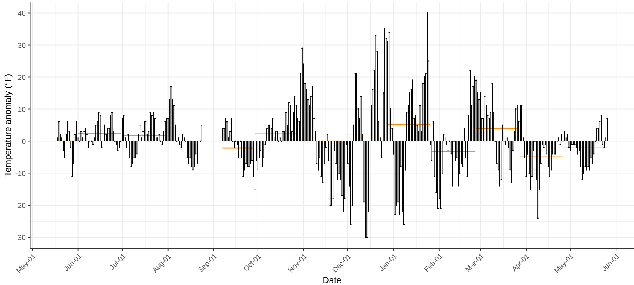
Difference between daily mean temperature and 30-year average, Fairbanks Airport (PAFA) 2021–2022
