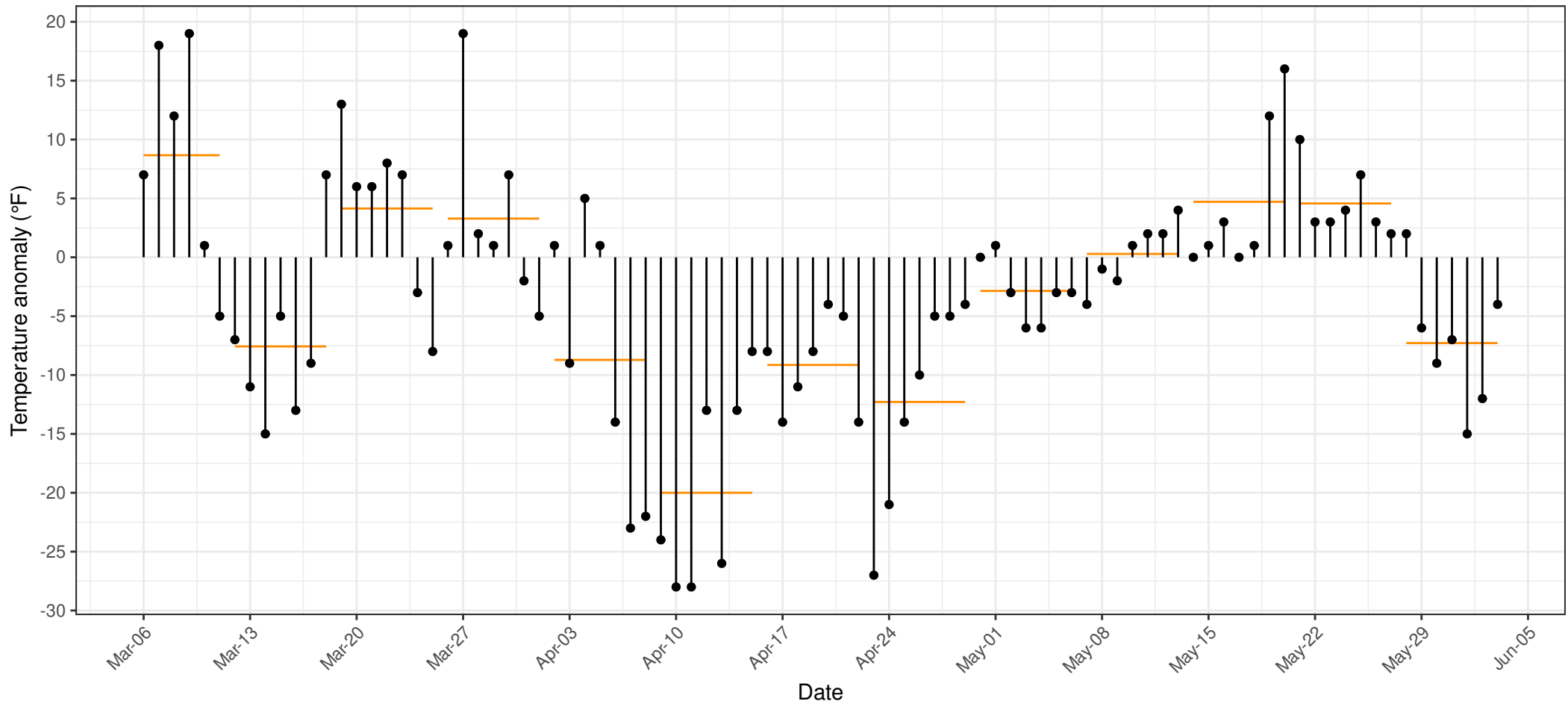
Difference between daily mean temperature and 30-year average, Fairbanks Airport (PAFA) 2023
